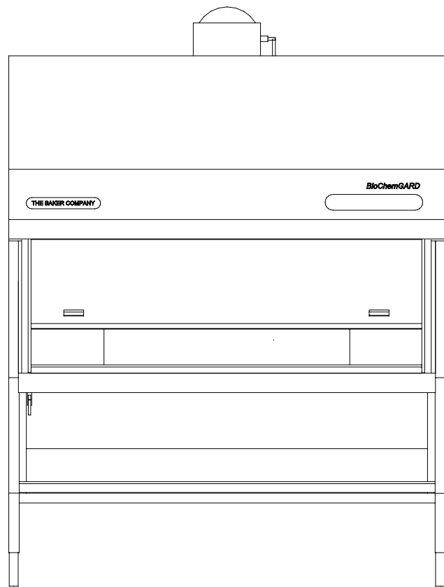
② FRONT VIEW 1/2" = 1'-0"
