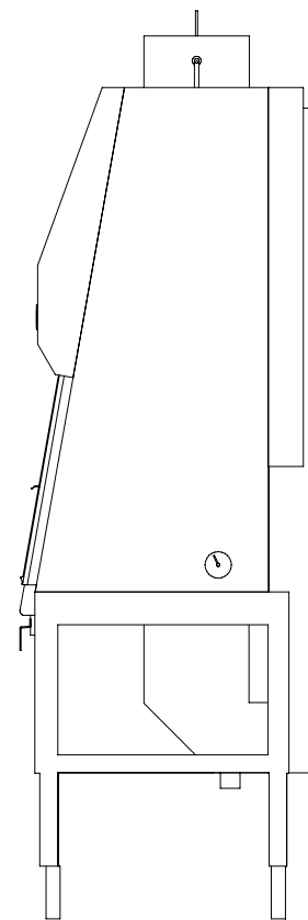
③ RIGHT VIEW 1/2" = 1'-0"
