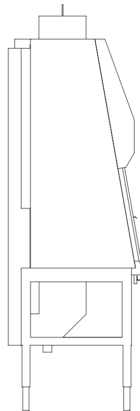
④ LEFT VIEW 1/2" = 1'-0"
